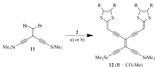
Scheme 2. Synthesis of TEE-extended TTF. a) [Pd(PhCN) 2 Cl 2 ], P( t Bu) 3 , CuI, HN( i Pr) 2 , THF, toluene, microwave heating, 60 °C, 6 min; 38%; b) [Pd(PhCN) 2 Cl 2 ], P( t Bu) 3 , CuI, HN( i Pr) 2 , THF, toluene, ultrasonication, 30 °C; 85%.
