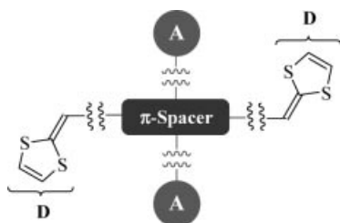
Figure 1. Schematic representation of extended TTF and donor–acceptor (D–A) dyads based hereupon.
