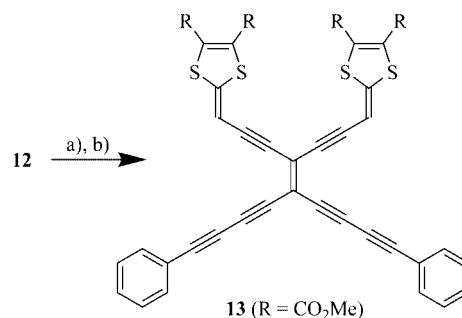
Scheme 3. Synthesis of extended TEE-TTF chromophore. a) K 2 CO 3 , THF, MeOH; b) phenylacetylene, CuCl, TMEDA, CH 2 Cl 2 , air; 18%. TMEDA = N,N,N',N' -tetramethylethylenediamine.
