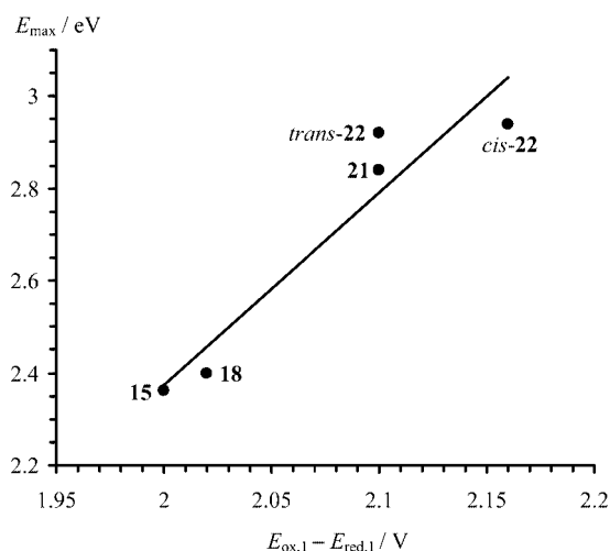
Figure 9. Correlation between optical and electrochemical HOMO–LUMO gaps for donor–acceptor molecules. E_{\text{max}} is the longest-wavelength absorption energy, E_{\text{ox},1} is the first oxidation potential, and E_{\text{red},1} is the first reduction potential.
