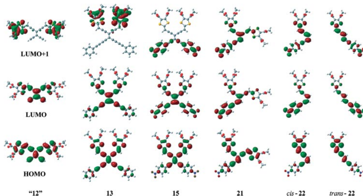
Figure 7. HOMO, LUMO, and LUMO+1 of 12 (Me 3 Si groups replaced by hydrogen atoms), 13 , 15 , 21 , cis - 22 , and trans - 22 calculated at the B3LYP/6-31+G(d) level.
