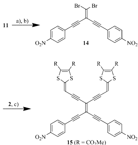
Scheme 4. Synthesis of donor-acceptor TEE. a) K 2 CO 3 , THF, MeOH; b) p -iodonitrobenzene, [PdCl 2 (PPh 3 ) 2 ], CuI, Et 3 N, THF; 54%; c) [Pd(PhCN) 2 Cl 2 ], P( t Bu) 3 , CuI, HN( i Pr) 2 , THF, toluene, ultrasonification, 30 °C; 97%.
