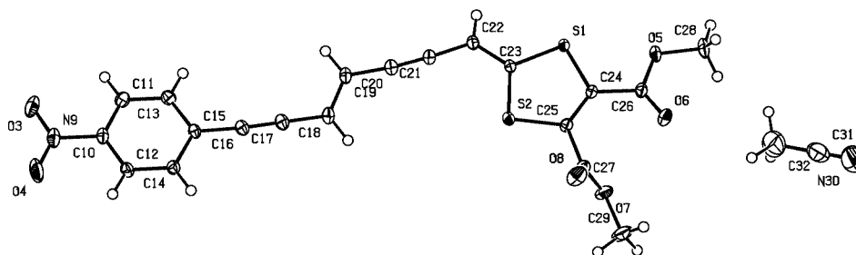
Figure 3. X-ray crystal structure of trans - 22 . All atoms of trans - 22 , except methyl hydrogens on C28 together with O7, O8 and the C29 methyl group, are almost planar (rmsd = 0.133 Å for 33 atoms). They make an angle of 65° with the plane formed by O7, O8, C25, C27 and C29 (rmsd = 0.009 Å). Drawing made by ORTEP-II. [34]
