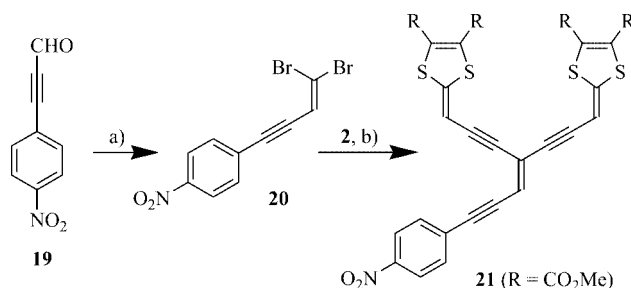
Scheme 6. Synthesis of donor-acceptor TriEE. a) CBr 4 , PPh 3 , Zn, CH 2 Cl 2 , room temp.; 72%; b) [Pd(PhCN) 2 Cl 2 ], P( t Bu) 3 , CuI, HN( i Pr) 2 , THF, toluene, ultrasonification, 30 °C; 30%.
