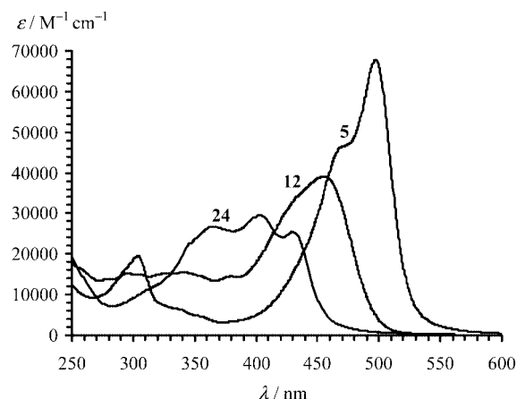
Figure 5. UV/Vis absorption spectra in CHCl 3 of extended TTFs.
