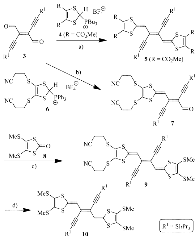
Scheme 1. Synthesis of DEE-extended TTFs. a) n BuLi, THF; 60%; b) NEt 3 , THF; 69%; c) P(OEt) 3 ; 79%; d) CsOH·H 2 O, MeI, THF, MeOH; 82%.
