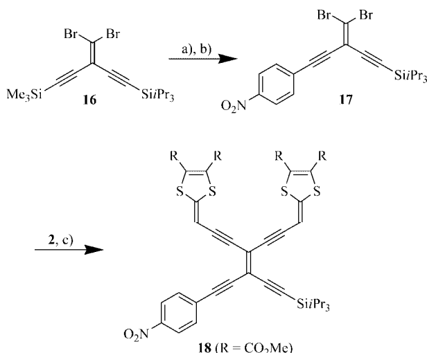
Scheme 5. Synthesis of unsymmetrical donor-acceptor TEE. a) K 2 CO 3 , THF, MeOH; b) p -iodonitrobenzene, [PdCl 2 (PPh 3 ) 2 ], CuI, Et 3 N, THF; 44%; c) [Pd(PhCN) 2 Cl 2 ], P( t Bu) 3 , CuI, HN( i Pr) 2 , THF, toluene, ultrasonification, 30 °C; 48%.
