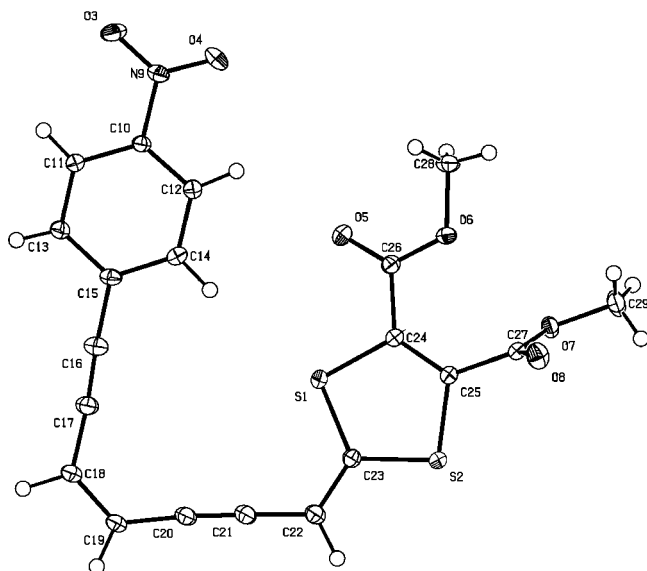
Figure 2. X-ray crystal structure of cis - 22 . All atoms, except methyl hydrogen atoms on C28 together with O7, O8 and the C29 methyl group, are approximately planar (rmsd = 0.206 Å for 33 atoms). They make an angle of 78° with the plane formed by O7, O8, C25, C27 and C29 (rmsd = 0.006 Å). Drawing made by ORTEP-II. [34]
