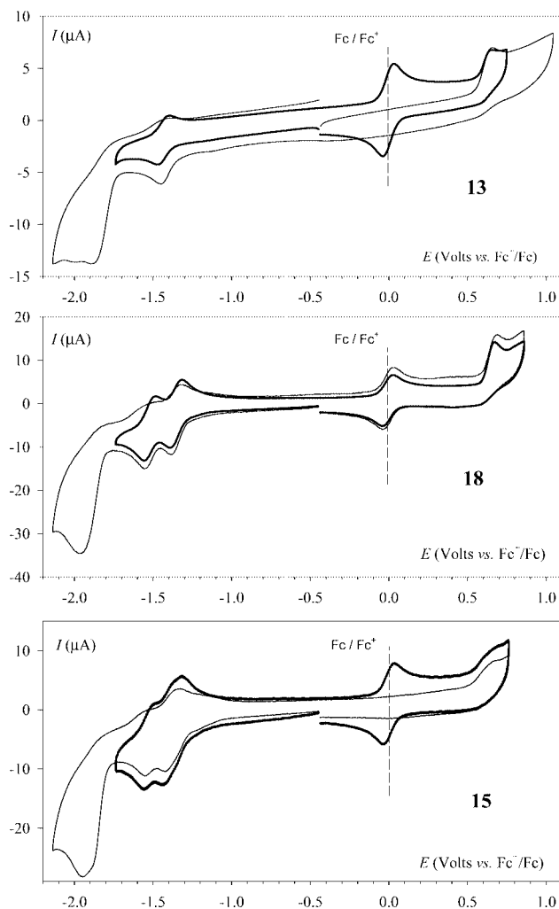
Figure 8. Cyclic voltammetry on a glassy carbon working electrode of compounds 13 , 15 , and 18 in \text{CH}_2\text{Cl}_2 + 0.1 M \text{Bu}_4\text{NPF}_6 . Scan rate: 0.1 \text{ V s}^{-1} .
