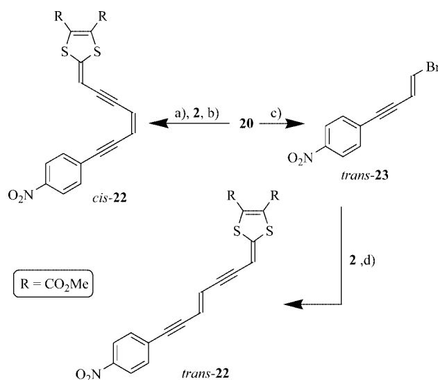
Scheme 7. Synthesis of donor-acceptor DEEs. a) [Pd(PPh 3 ) 4 ], Bu 3 SnH, toluene; b) CuI, HN( i Pr) 2 , THF; 39%; c) HPO(OEt) 2 , Et 3 N, 50 °C; 42%; d) [Pd(PPh 3 ) 4 ], CuI, HN( i Pr) 2 , toluene, THF; 67%.
