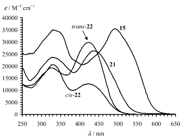
Figure 6. UV/Vis absorption spectra in CHCl 3 of donor-acceptor molecules.
